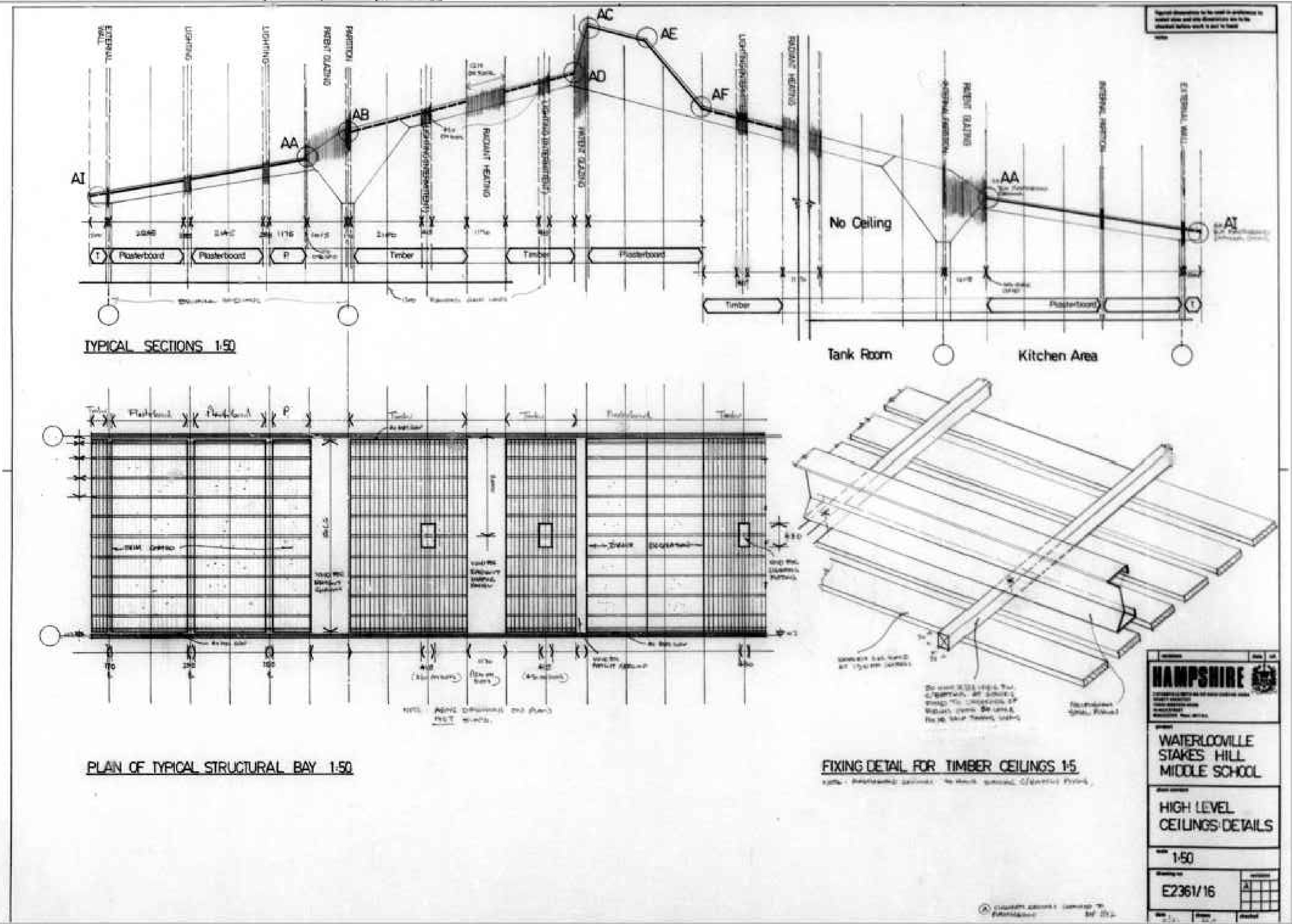
2 Original details of the existin ceiling details
