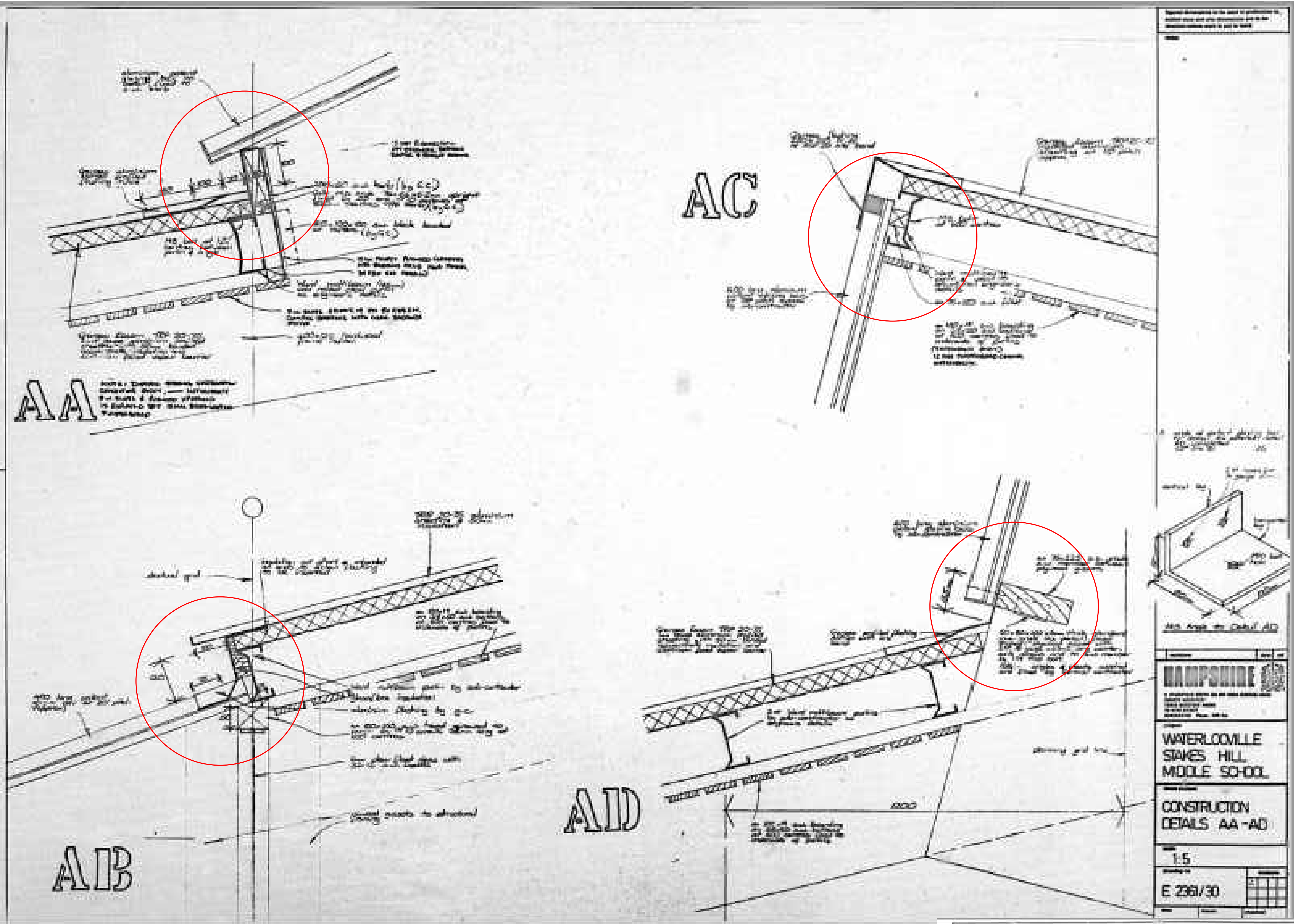
1 Original details of the existing patent glazing
