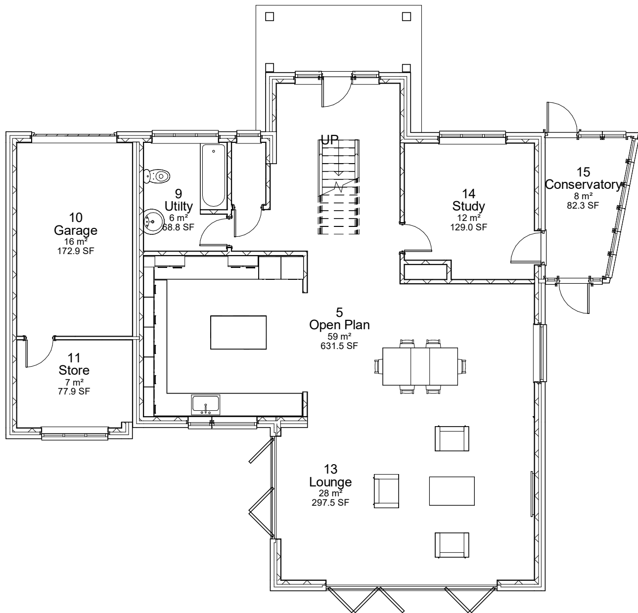
1 Ground Floor Plan
