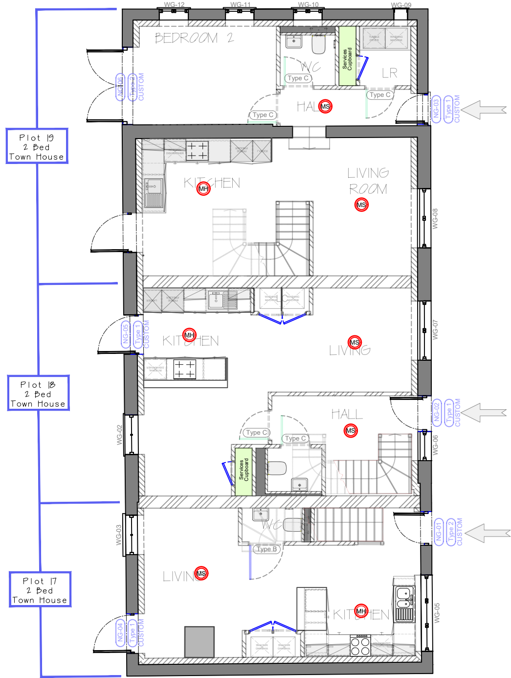
Former Coach House - Ground Floor [Building Control Layout] Scale 1:100@A1
