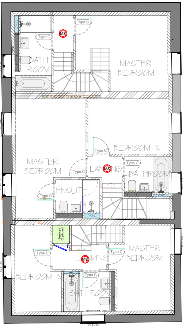
Former Coach House - First Floor [Building Control Layout] Scale 1:100@A1
