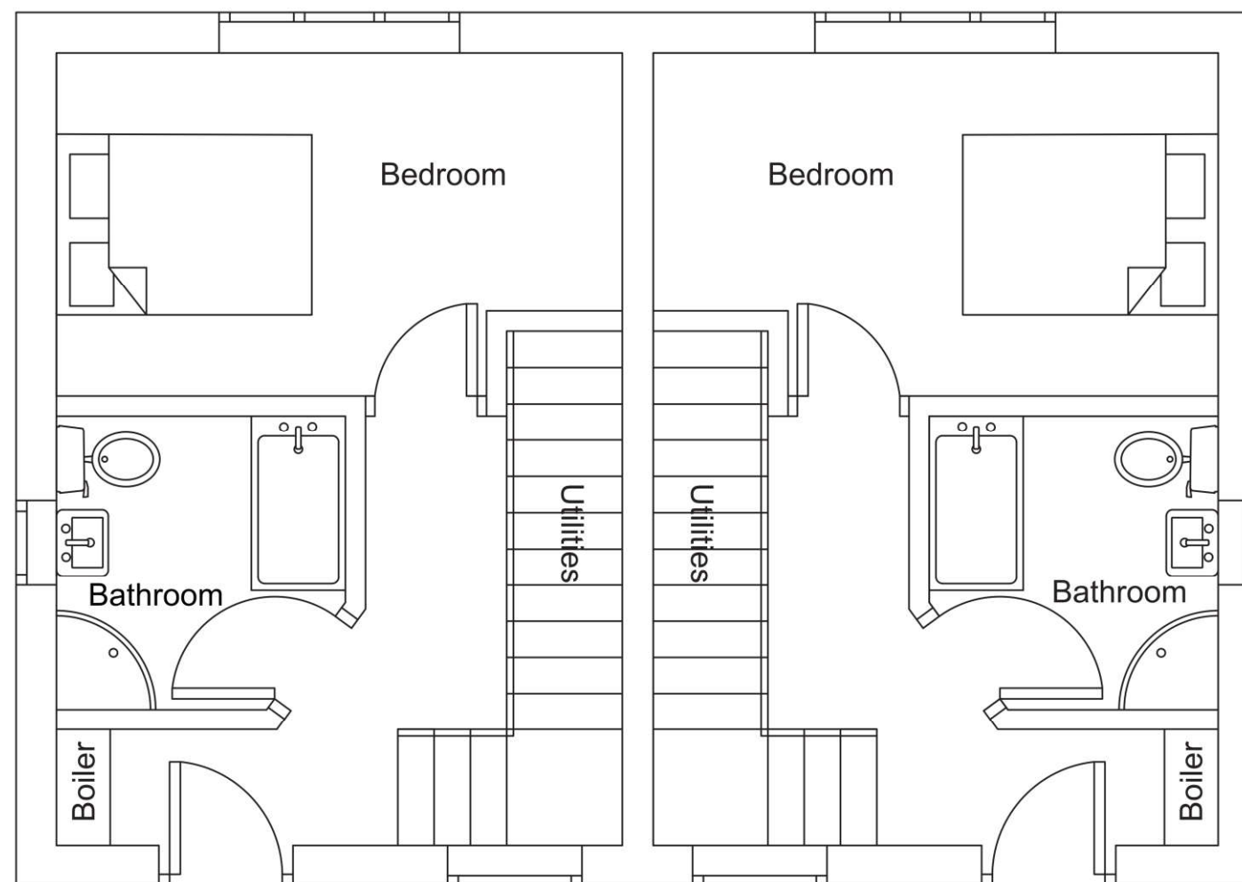
Proposed Ground Floor Layout
