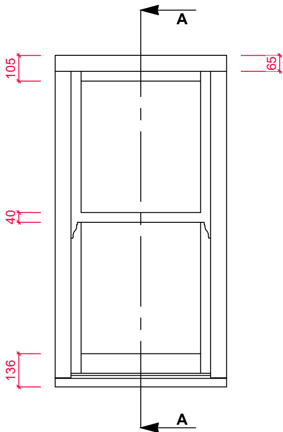
TYPICAL 65mm-FRAME LAYOUT WITH TOP SASH HORNS 65mm FRAME ONLY AVAILABLE ON FIXED SASHES
