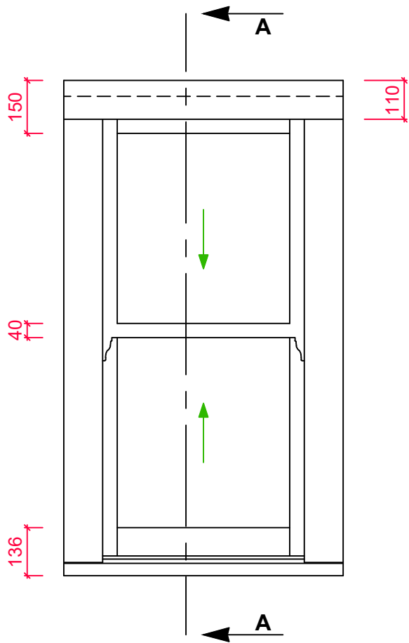
TYPICAL 110mm-FRAME LAYOUT WITH TOP SASH HORNS REDUCED 65mm FRAME HEAD ALSO AVAILABLE
