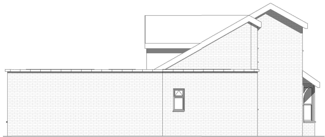
Proposed Elevation-Right side
