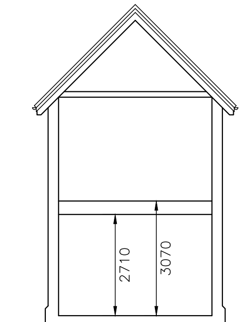
Section B-B
