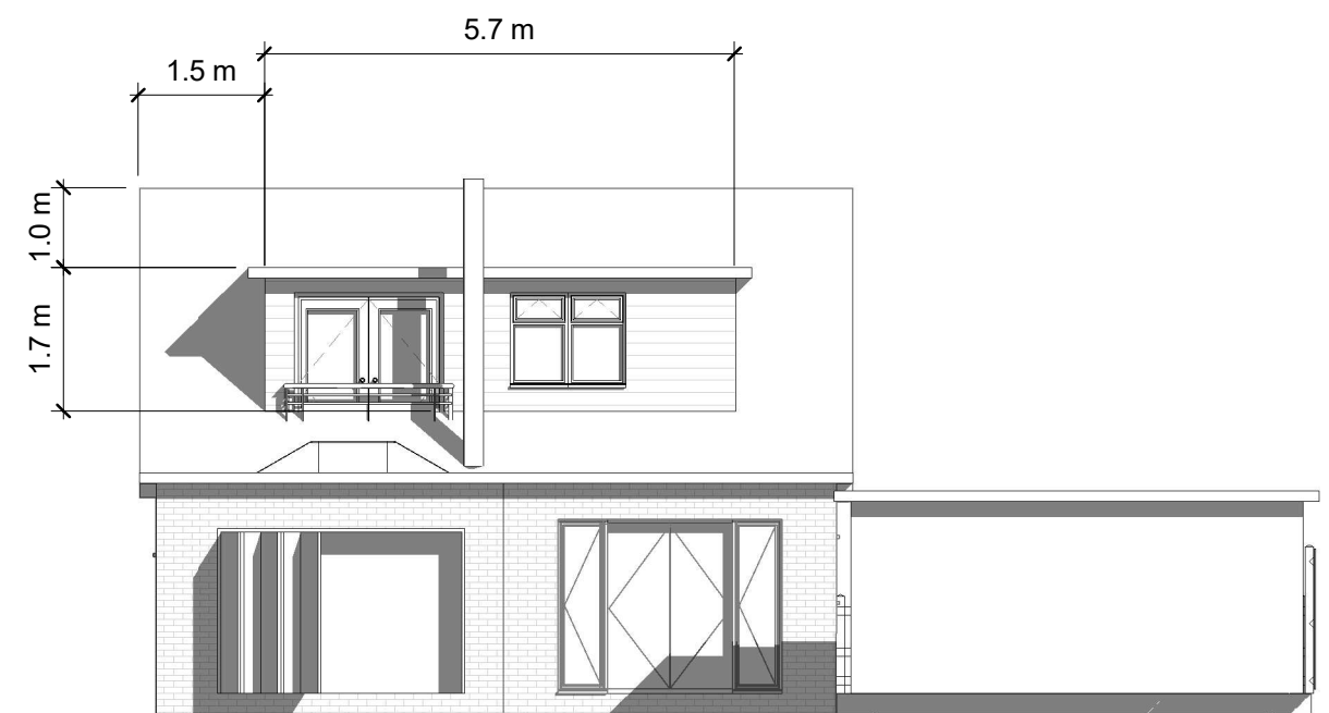
Proposed Elevation-Rear
