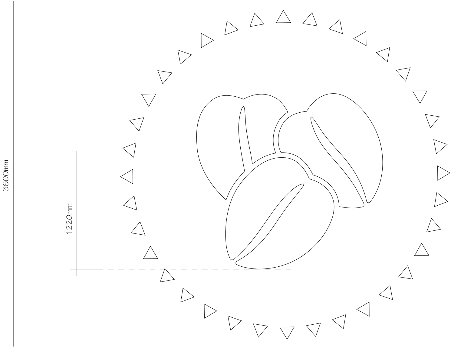
CUT OUT THREE BEAN 3600mm DIAMETER x 2mm POWDER COATED ALUMINIUM. FIXED TO WALL USING PINS TO BACKS OF ALUMINIUM. Scale 1:25
