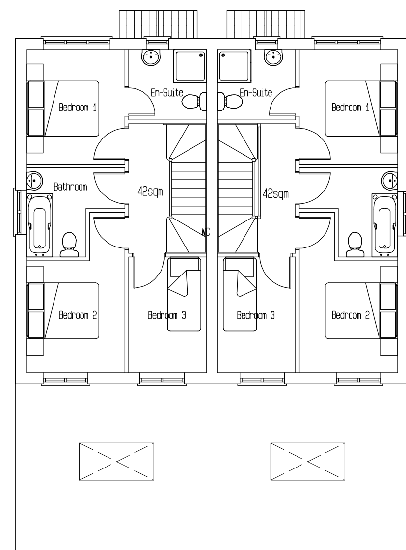
First Floor Plan Plots 1 & 2
