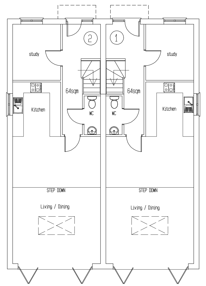
Ground Floor Plan Plots 1 & 2
