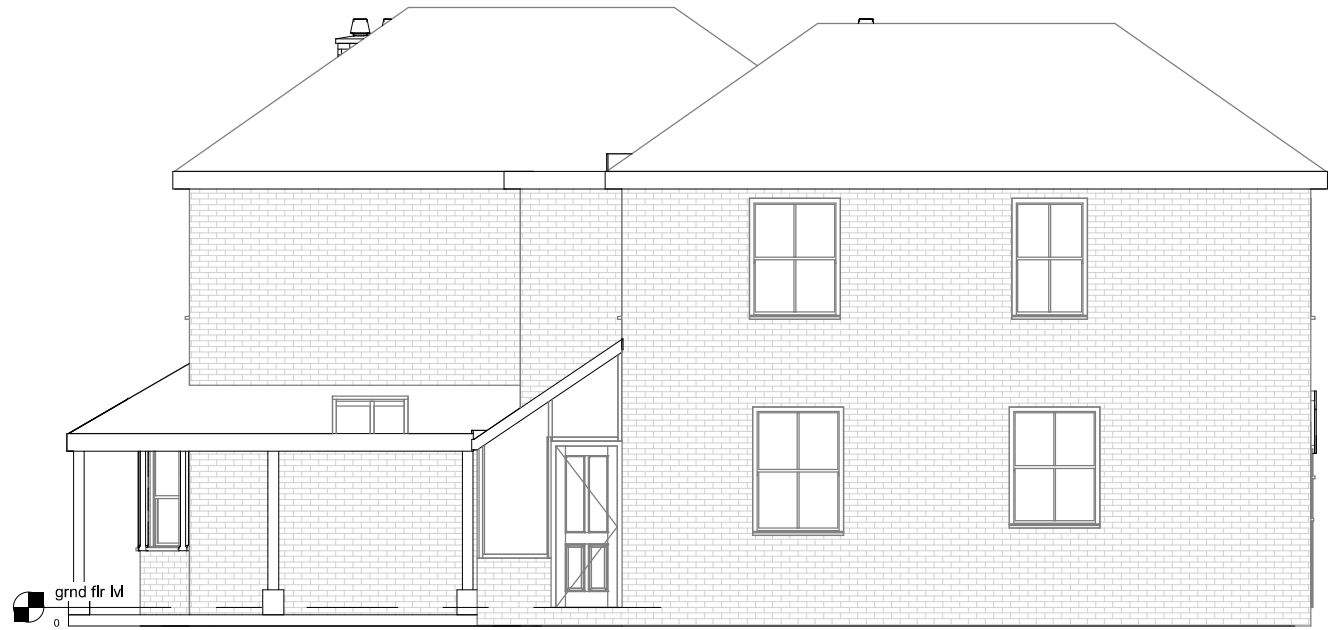
Existing Elevation-Right side
