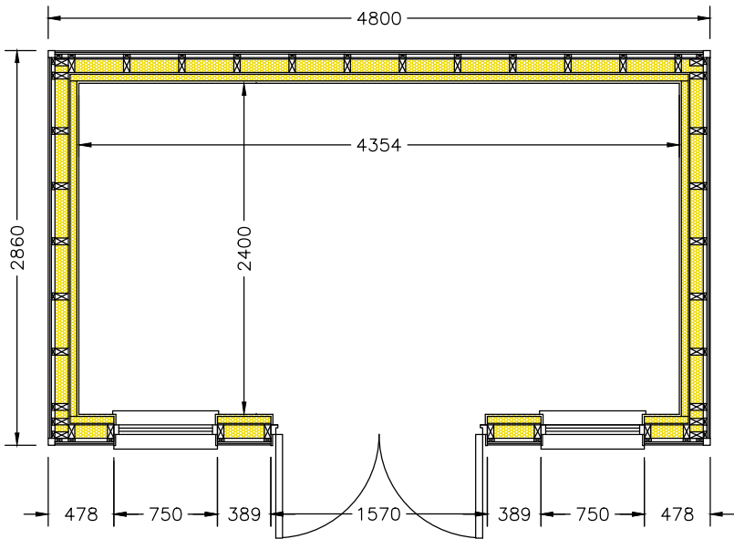
Proposed Plan (1:50)
