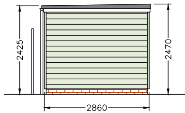
Proposed West Elevation (1:100)
