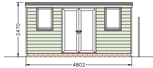
Proposed South Elevation (1:100)
