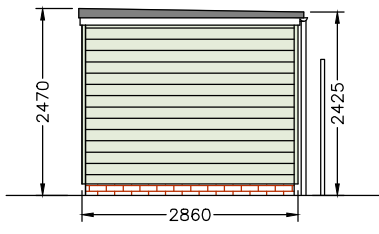
Proposed East Elevation (1:100)
