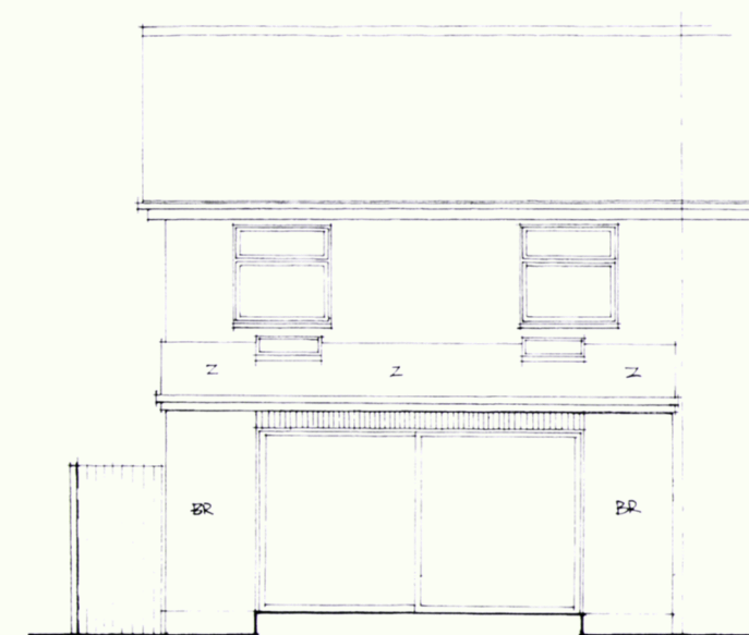
EAST ELEVATION
