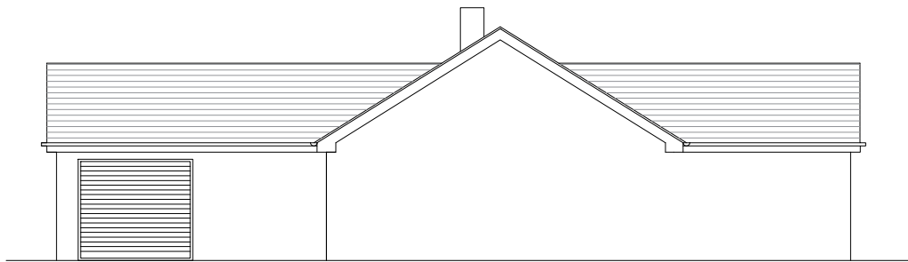
SIDE ELEVATION (East)
