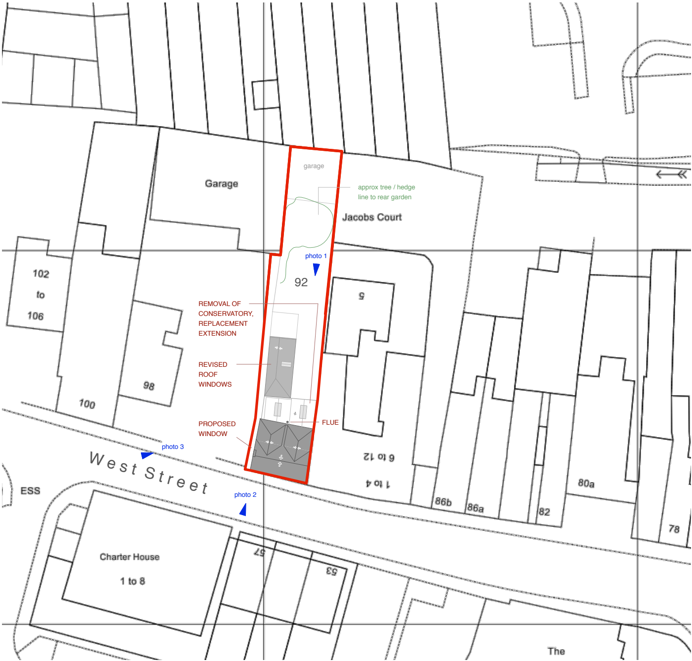
Proposed Site Plan at 1:500 scale
