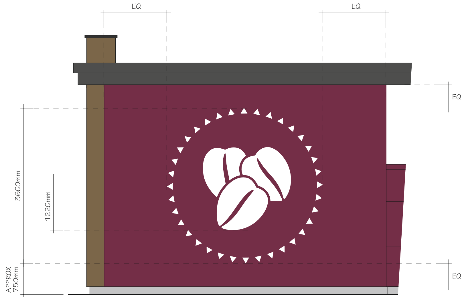
CUT OUT THREE BEAN 3600mm DIAMETER x 2mm POWDER COATED ALUMINIUM. FIXED TO WALL USING PINS TO BACKS OF ALUMINIUM. Scale 1 : 50
