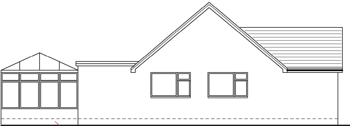
left (north west) elevation
