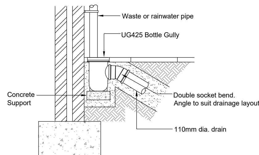
Bottle gully detail
