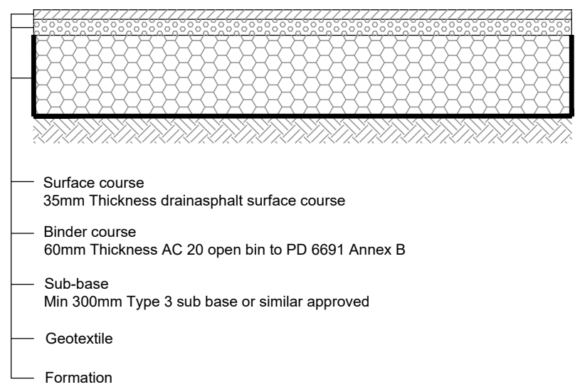
Permeable asphalt construction (Tanked)
