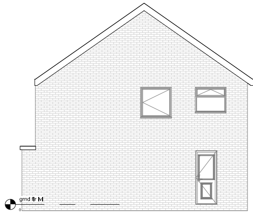
Existing Elevation-Right side
