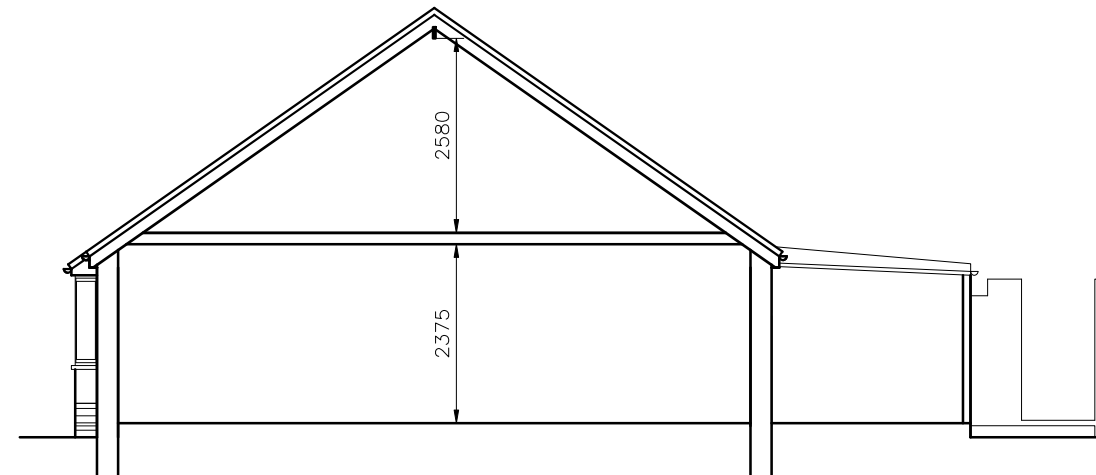
NORTH/ DRAFT SECTION
