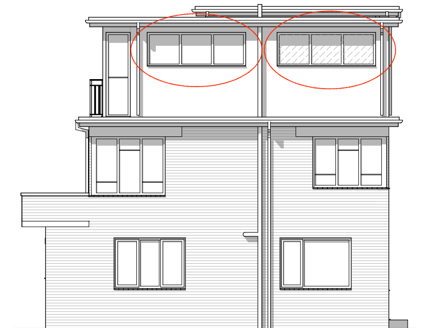
Proposed Side (N) Elevation 1:100
