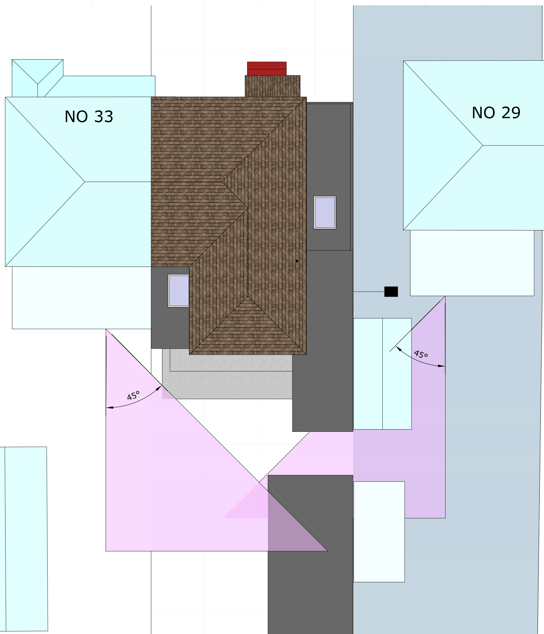
45 DEGREE PLAN GROUND FLOOR WINDOWS
