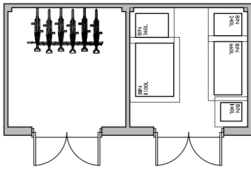
FLOOR PLAN
