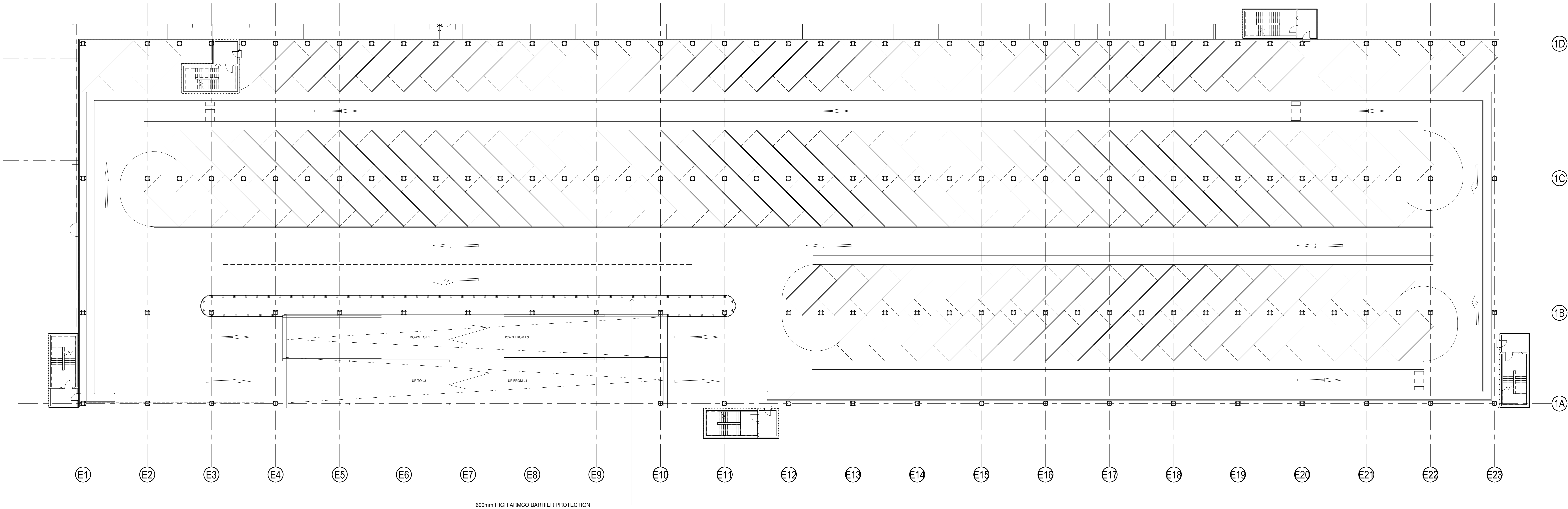
VAN PARKING DECK LEVEL - 4200 AFFL 1 : 200
