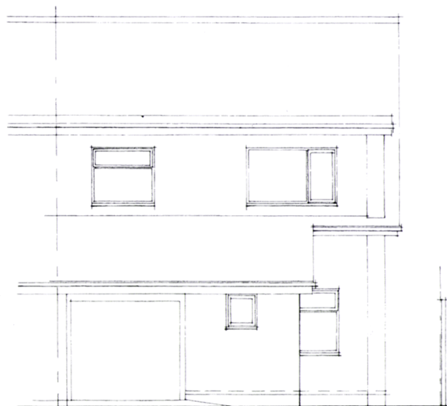
WEST ELEVATION
