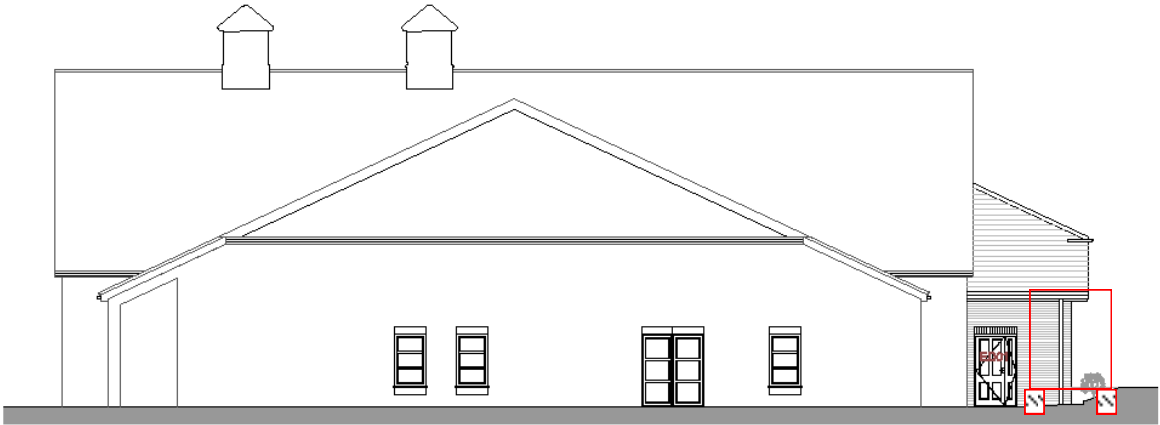
East Elevation
