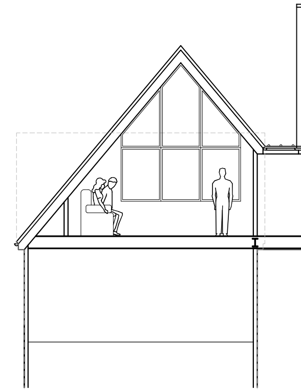
Transverse Section
