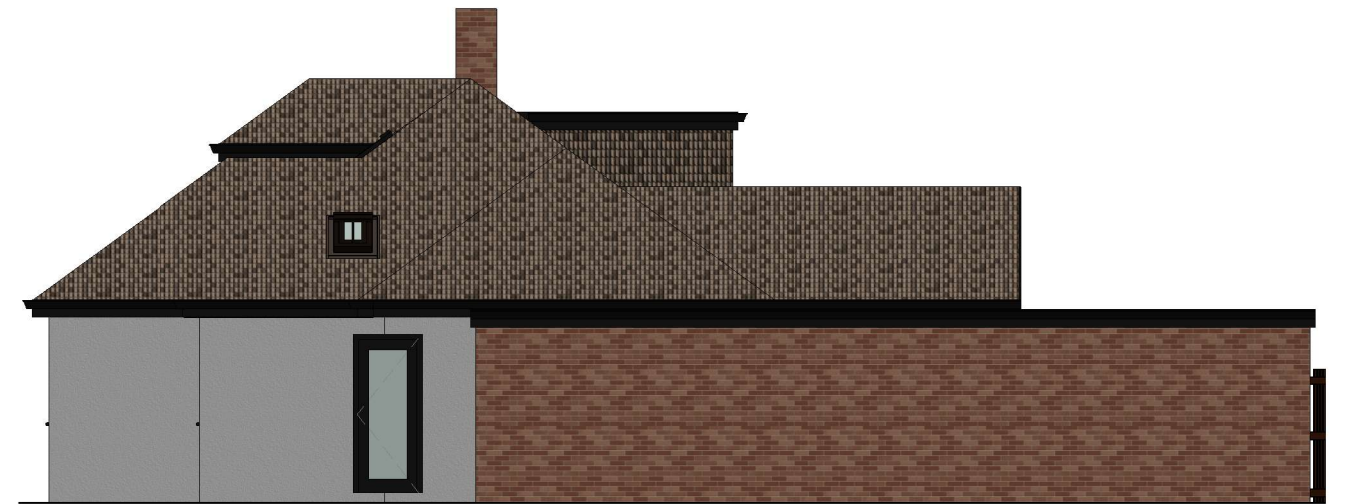
2 North Elevation 1 : 100
