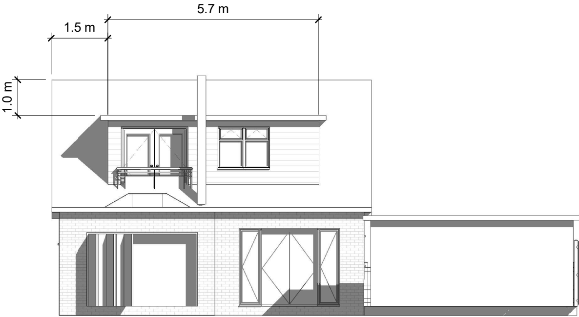
Proposed Elevation-Rear
