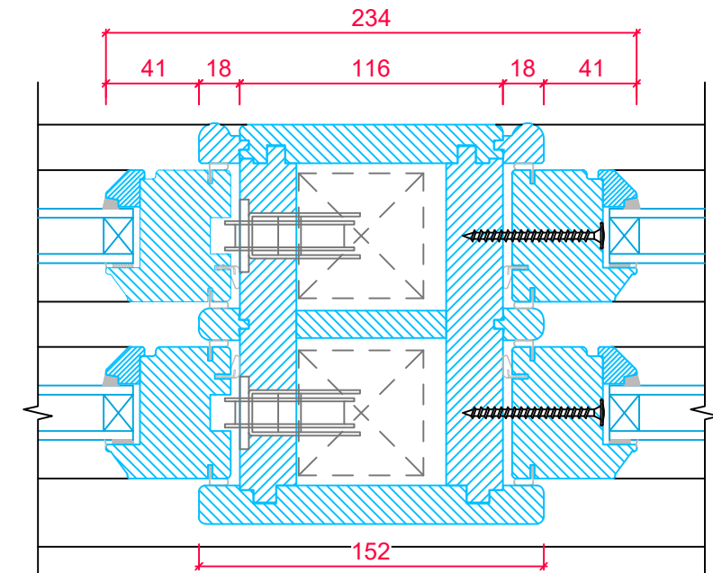
CENTRAL MULLION FOR DOUBLE OPENING FIXED COMBO SASH
