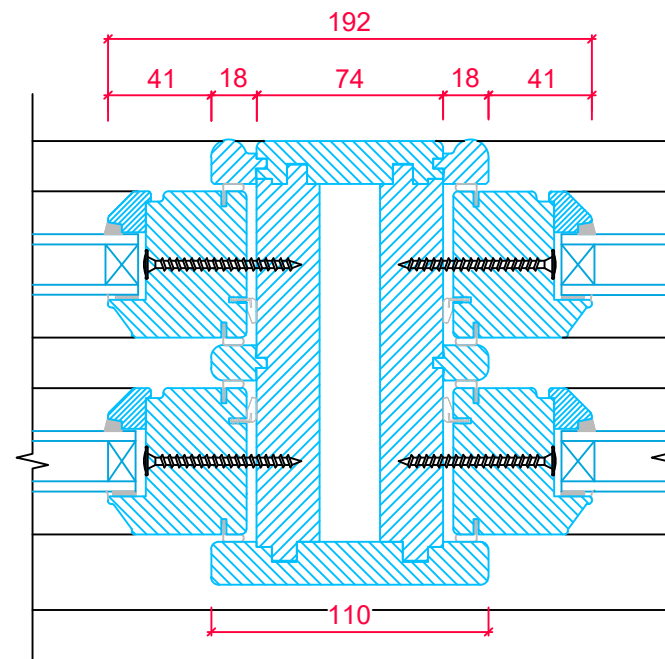
CENTRAL MULLION FOR DOUBLE FIXED SASH
