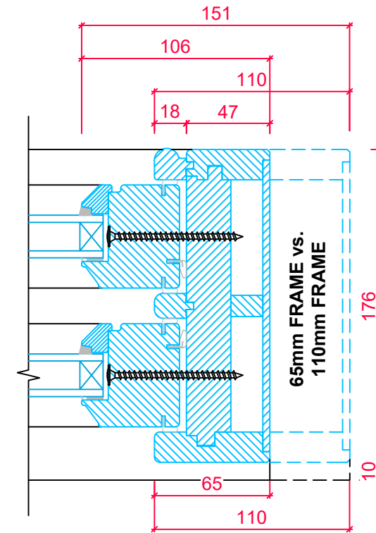
RH JAMB SECTION FOR FIXED SASH (LH IS DIRECT MIRROR)
