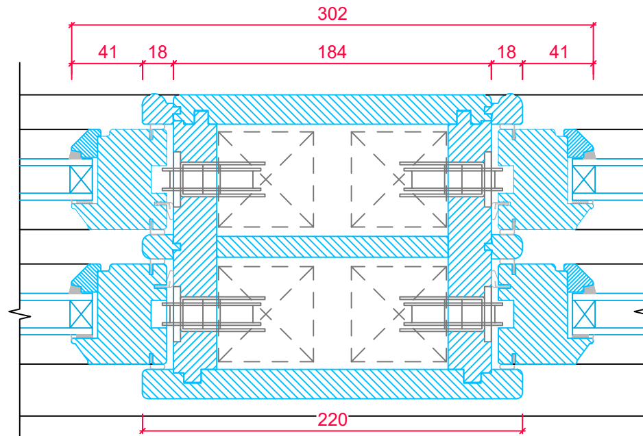
CENTRAL MULLION FOR DOUBLE OPENING SASH (both sashes open independently)
