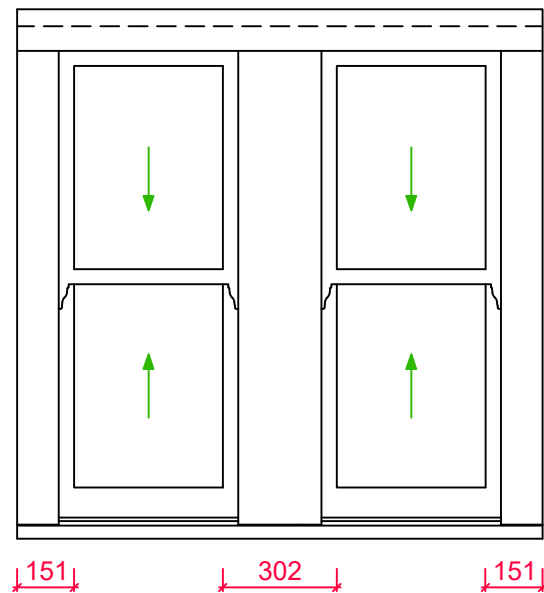
TYPICAL DOUBLE OPENING SASH LAYOUT
