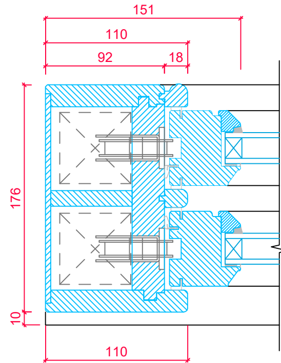
LH JAMB SECTION FOR OPENING SASH (RH IS DIRECT MIRROR)
