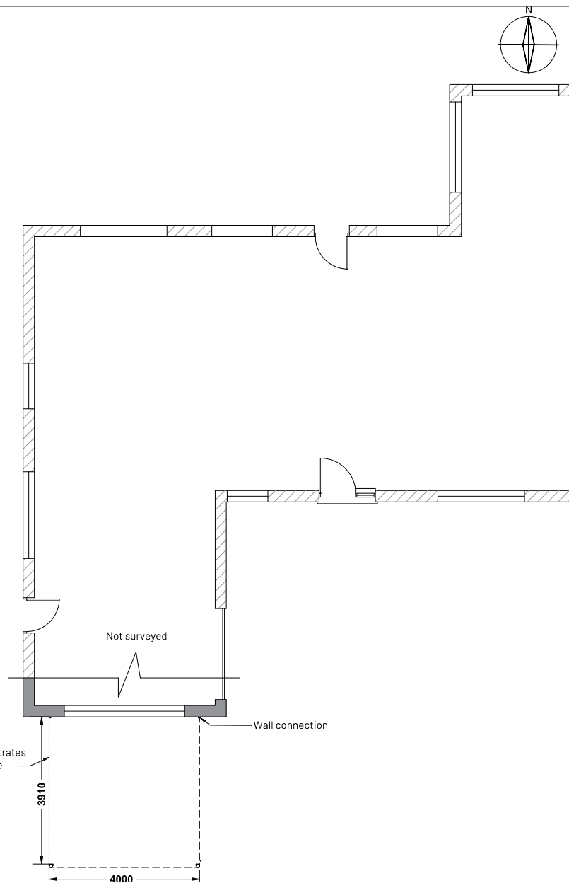
FLOOR PLAN
