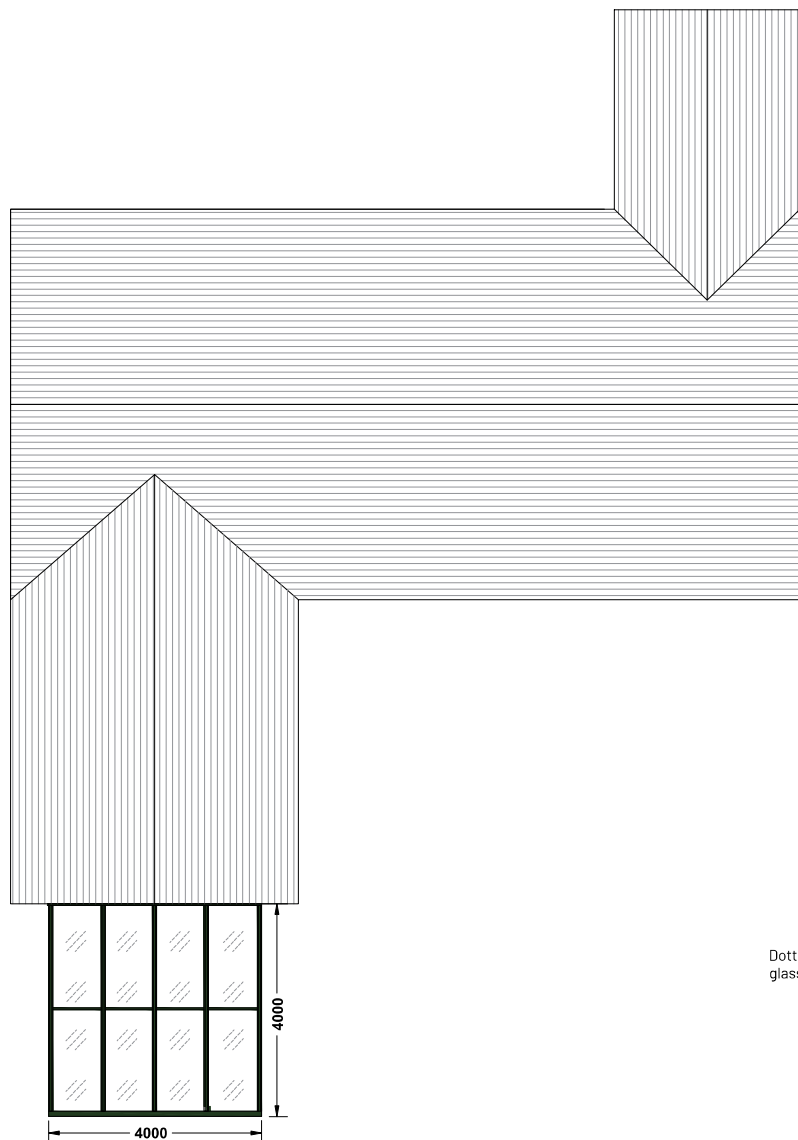
ROOF PLAN
