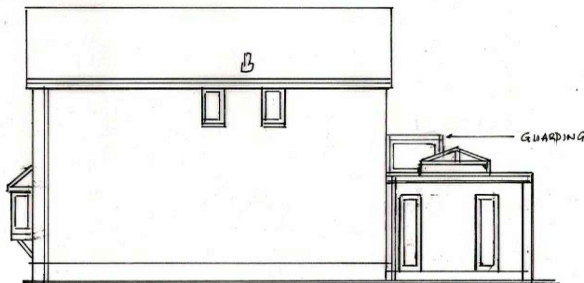
SIDE (EAST)
