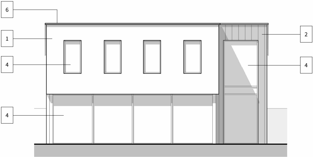
1 North Elevation - 1 : 100
