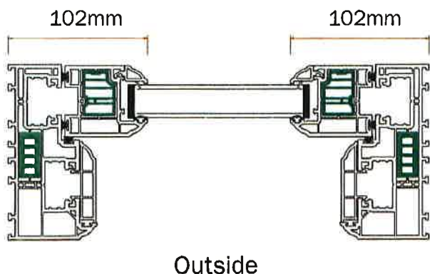
Horizontal Section Through Bottom Sash
