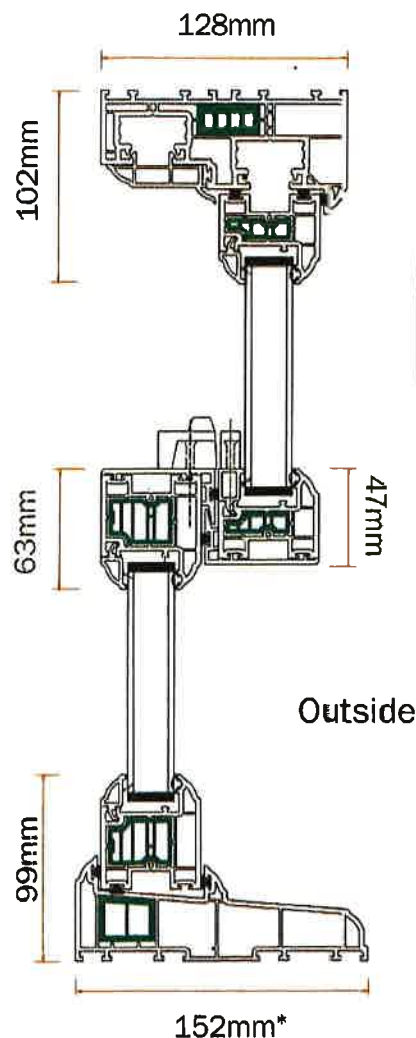
Vertical Section Through Sash
