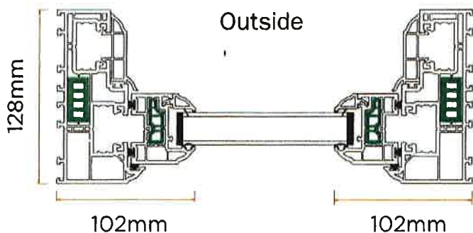
Horizontal Section Through Bottom Sash
