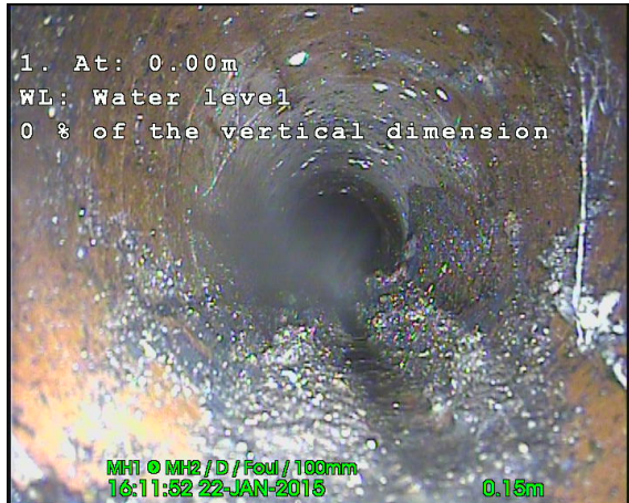
Photo: 150122_1611C-Survey.jpg 0.31m, Water level 0 % of the vertical dimension
