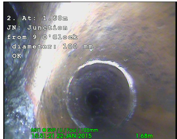
Photo: 150122_1551A-Survey.jpg 1.71m, Junction from 9 O'Clock diameter: 100 mm OK
