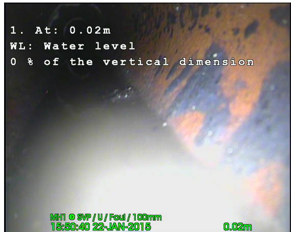
Photo: 150122_1550C-Survey.jpg 0.04m, Water level 0 % of the vertical dimension
