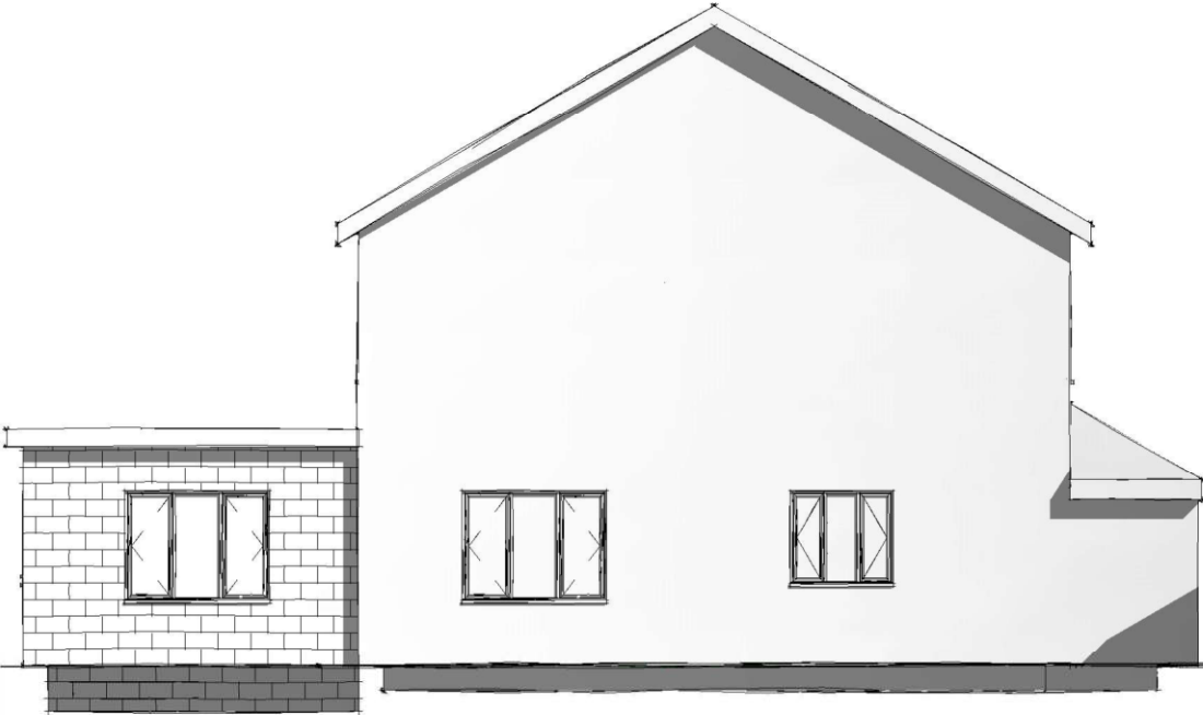
West Elevations Proposed
