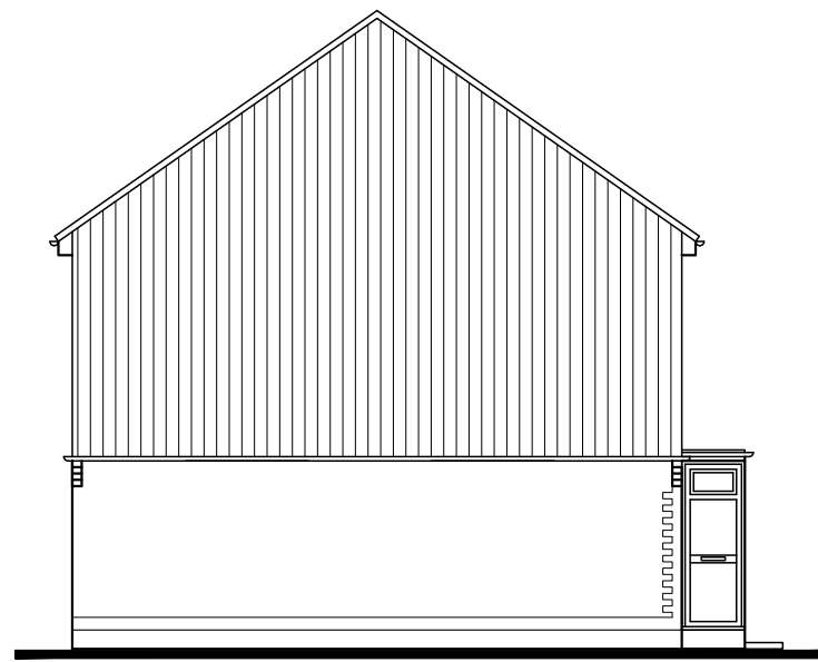
South Elevation
