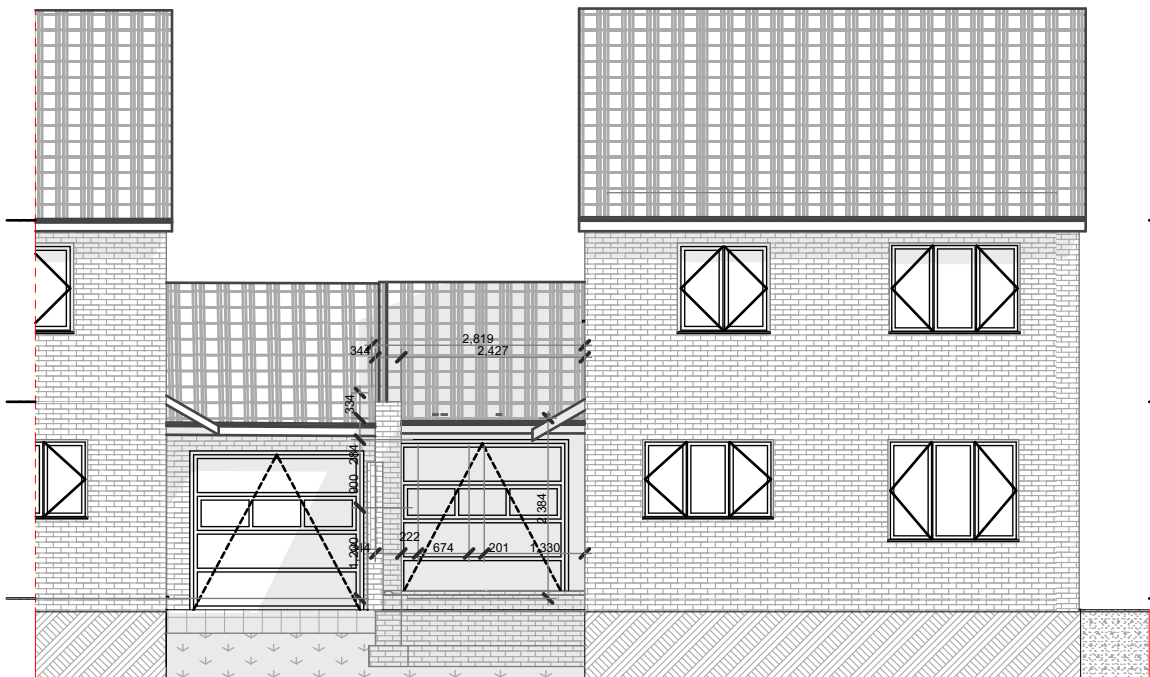
EAST ELEVATION 1:100
