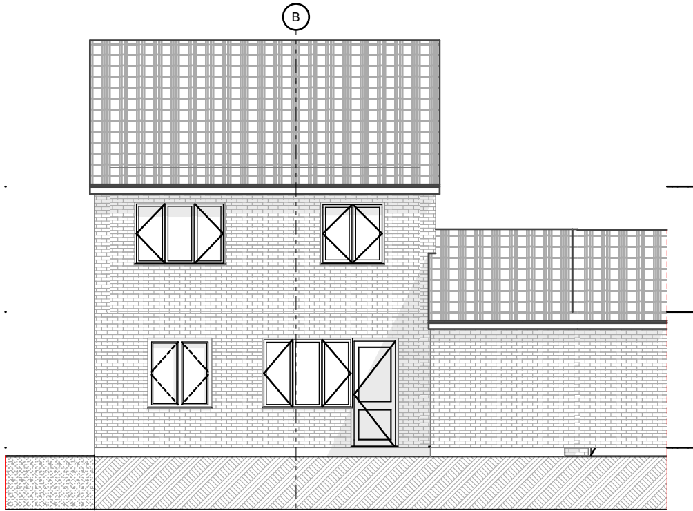
WEST ELEVATION 1:100
