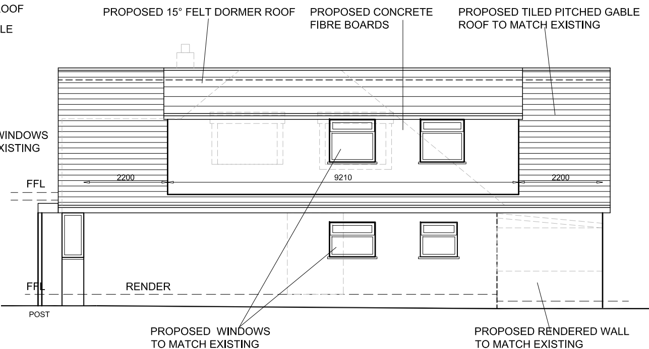
EAST ELEVATION R/H ELEVATION
