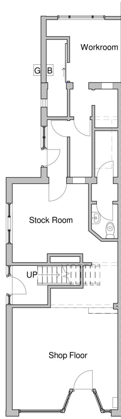
Existing Ground Floor 1 : 100
