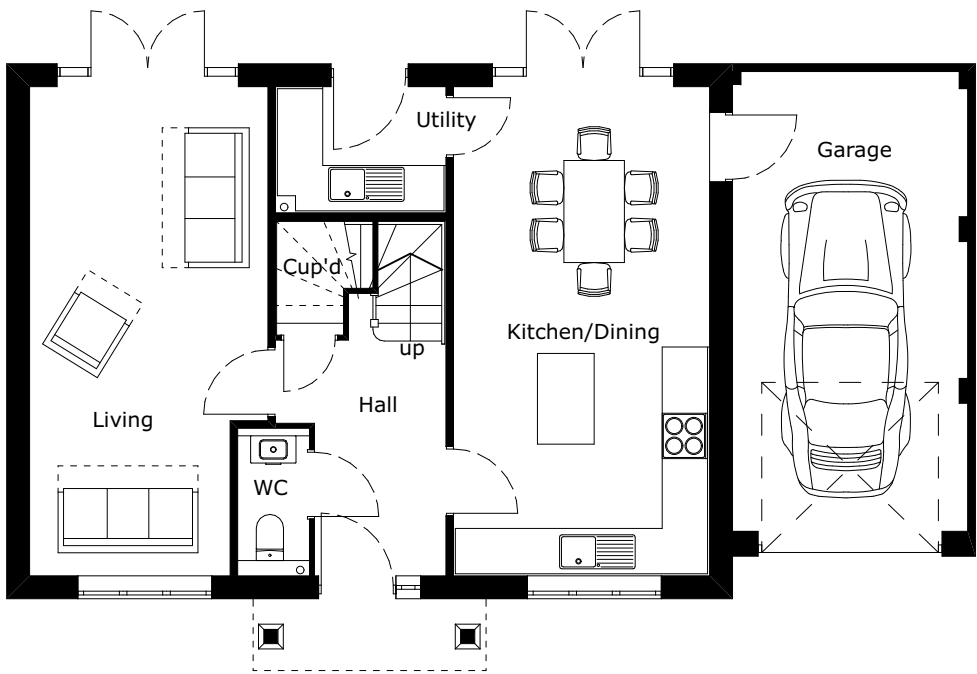
GROUND FLOOR - 1:100
