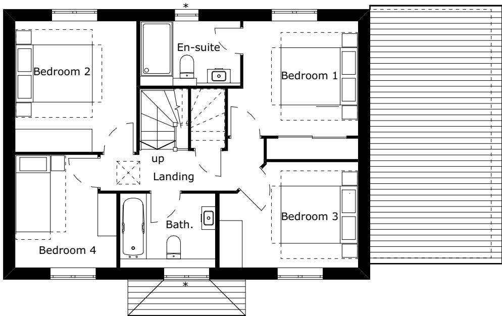
FIRST FLOOR - 1:100
