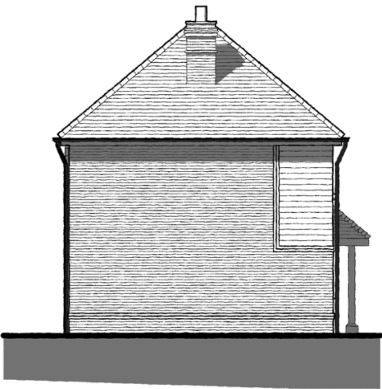
SIDE ELEVATION [2] - 1:100
