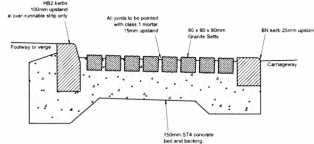
TYPICAL OVER-RUNNABLE STRIP (Scale 1:10)
