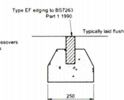
FLAT TOP EF EDGING DETAIL (Scale 1:10)
