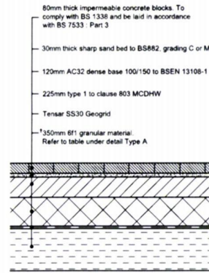
TYPE B - BLOCK PAVING CARRIAGEWAY CONSTRUCTION (Scale 1:20)
