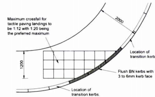
TYPICAL TACTILE PAVING LAYOUT (Scale 1:20)
