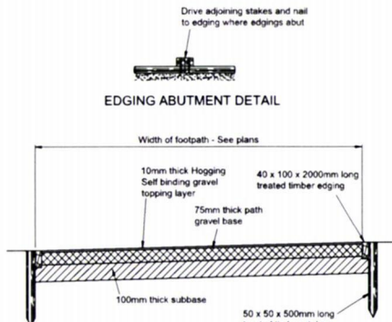
TYPE J - RURAL FOOTPATH (Scale 1:20)
