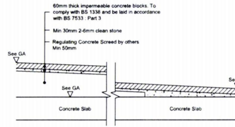
TYPE D - BLOCK PAVING UNDERCROFT VEHICLE ACCESS CONSTRUCTION DETAIL PLOTS 16 AND 37-41 (Scale 1:20)
