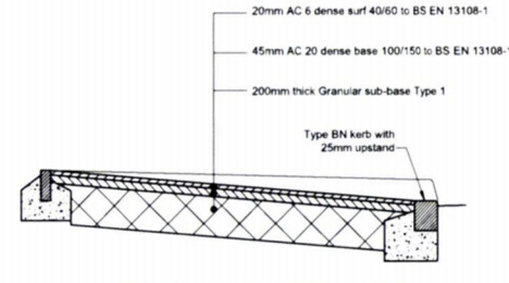
TYPE H - ASPHALT CONCRETE VEHICULAR CROSSOVER CONSTRUCTION (Scale 1:20)
