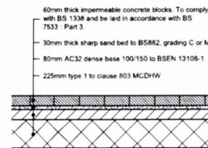
TYPE C - BLOCK PAVING DRIVE CONSTRUCTION (Scale 1:20)
