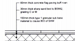
TYPE K - PAVING SLAB PATIO / FOOTPATH CONSTRUCTION (Scale 1:20)
