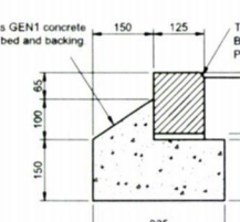
BN KERB DETAIL (Scale 1:10)
