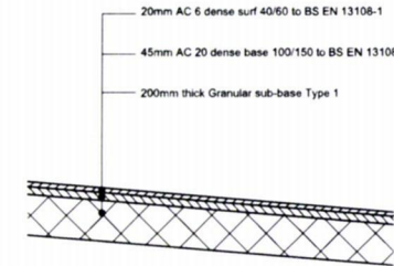
TYPE E - ASPHALT CONCRETE DRIVEWAY CONSTRUCTION (Scale 1:20)
