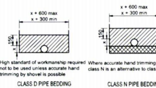
CLASS D PIPE BEDDING
