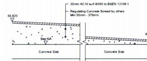
TYPE F - TARMAC UNDERCROFT VEHICLE ACCESS CONSTRUCTION DETAIL - PLOT 16 (Scale 1:20)
