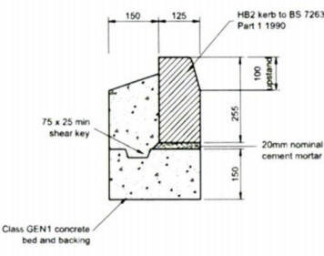
HB2 KERB DETAIL (Scale 1:10)
