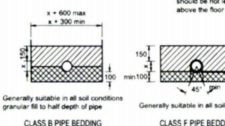
CLASS B PIPE BEDDING
