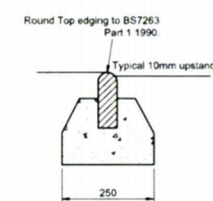
ROUND TOP EDGING DETAIL (Scale 1:10)
