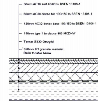
TYPE A - ASPHALT CONCRETE CARRIAGEWAY CONSTRUCTION (Scale 1:20)
