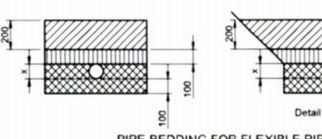
PIPE BEDDING FOR FLEXIBLE PIPES
