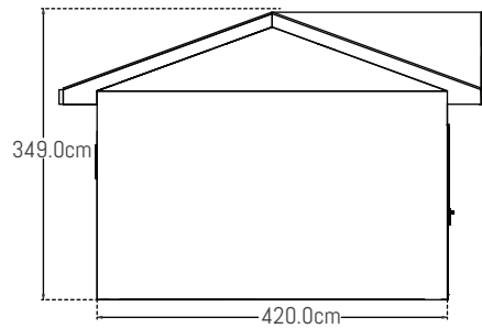
Left elevation
