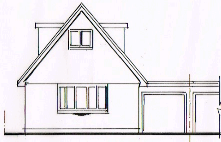
FRONT (EAST)
