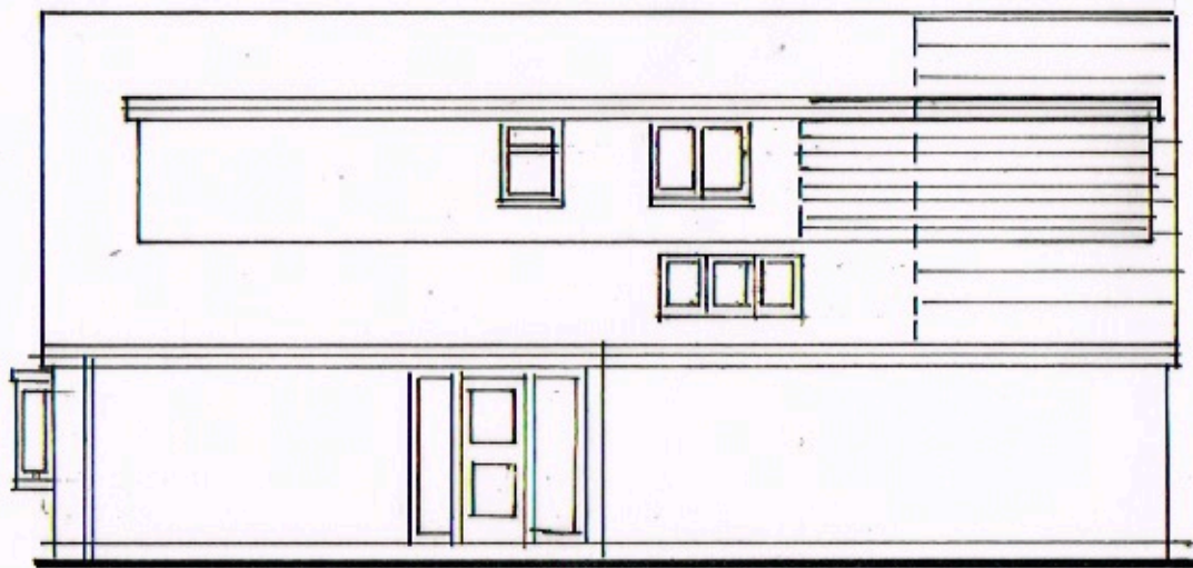
SIDE (NORTH)
