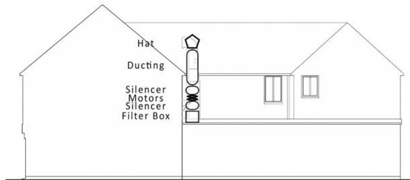
8 South Elevation (Existing & Proposed) Scale: 1:100
