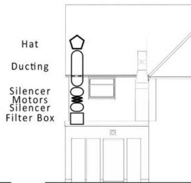
7 East Elevation (Existing & Proposed) Scale: 1:100
