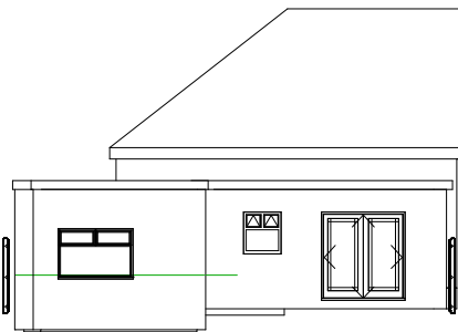
Existing South Elevation (Rear)
