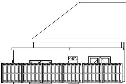
Proposed South Elevation (Rear)
