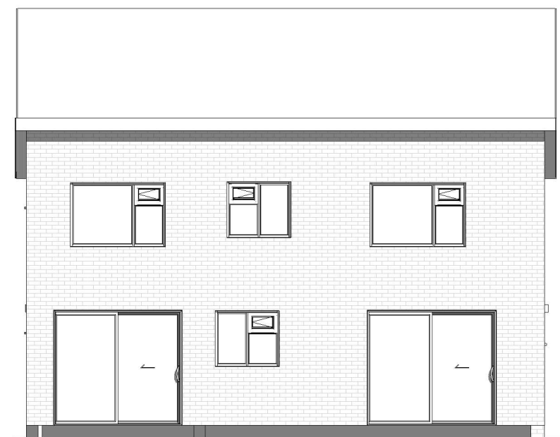
Proposed Elevation-Rear
