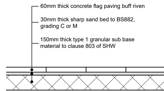
TYPE E - PAVING SLAB PATIO / FOOTPATH CONSTRUCTION (Scale 1:20)
