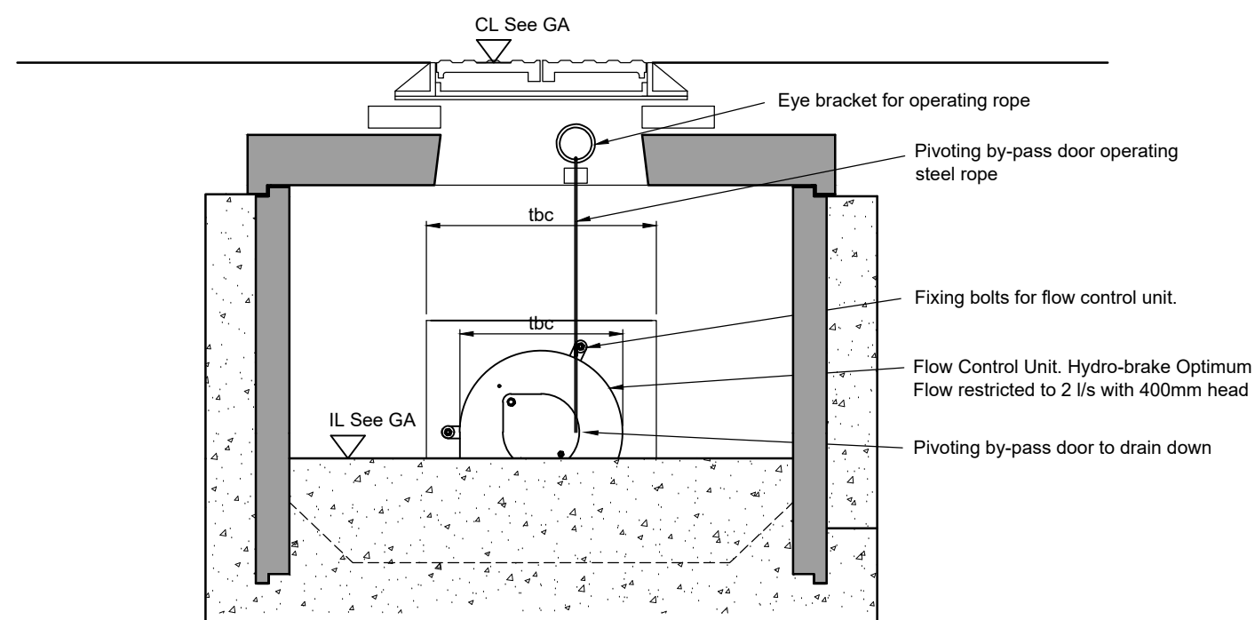
SECTION (Scale 1:20)
