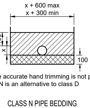
CLASS N PIPE BEDDING
