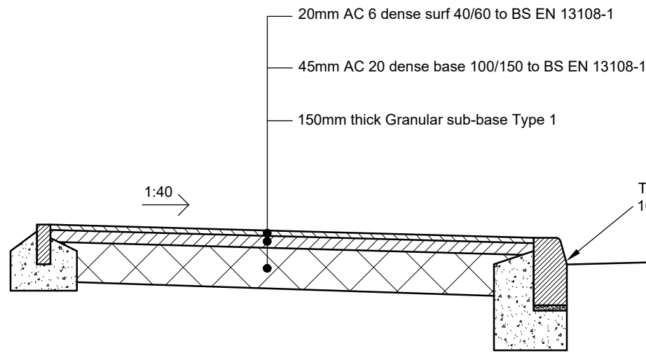
TYPE C - ASPHALT CONCRETE FOOTWAY CONSTRUCTION (Scale 1:20)
