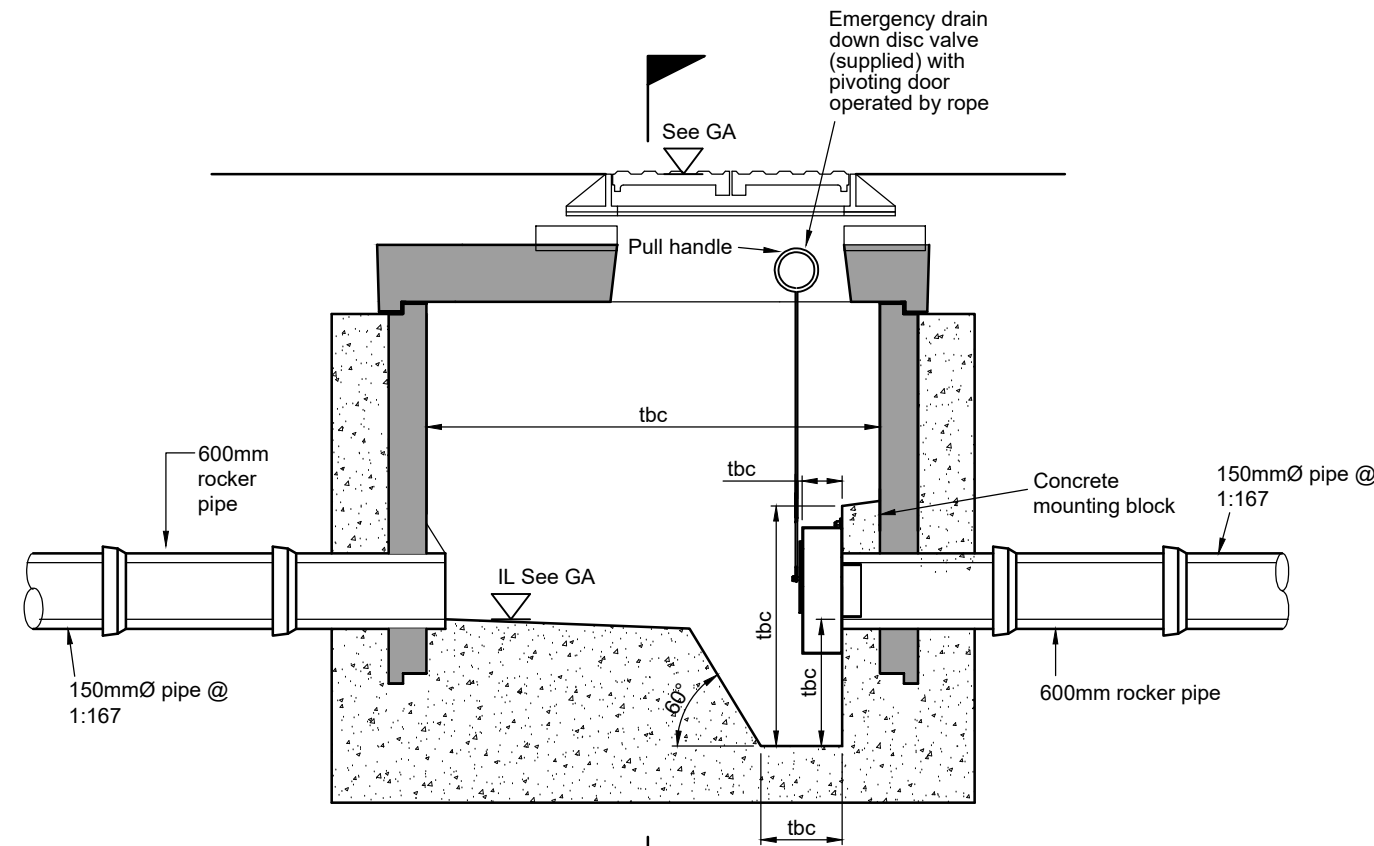
SECTION (Scale 1:20)
