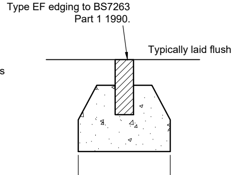
EF EDGING DETAIL (Scale 1:10)
