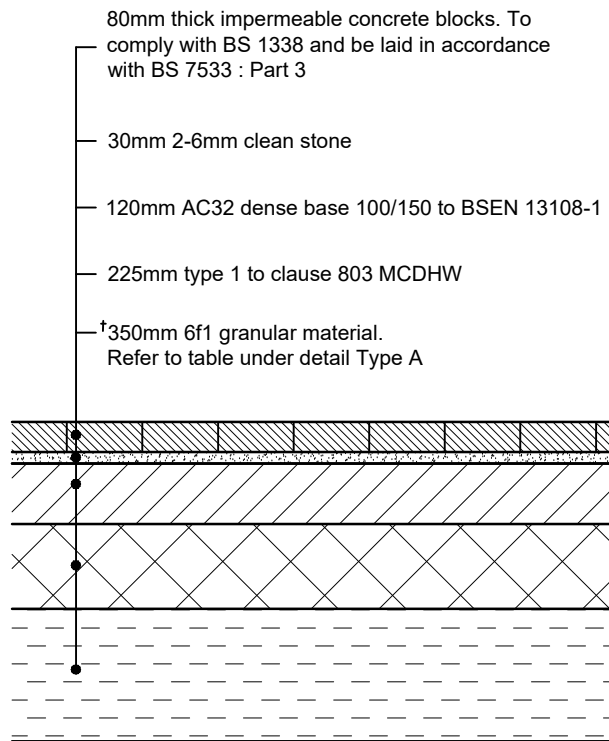
TYPE B - BLOCK PAVING CARRIAGEWAY CONSTRUCTION (Scale 1:20)
