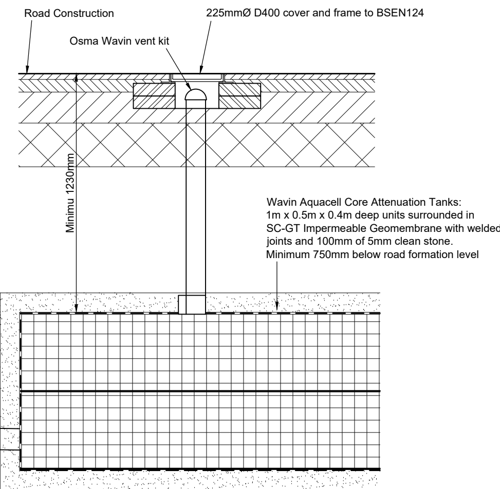
OSMA WAVIN AQUACELL STORAGE TANK DETAIL (Scale 1:20)
