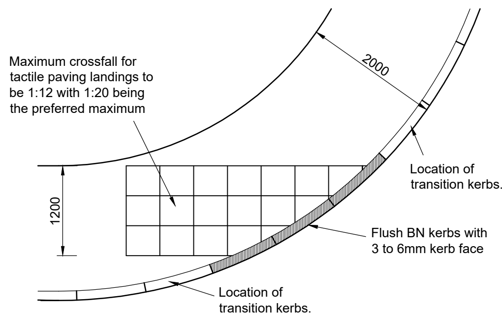
TYPICAL TACTILE PAVING LAYOUT (Scale 1:20)
