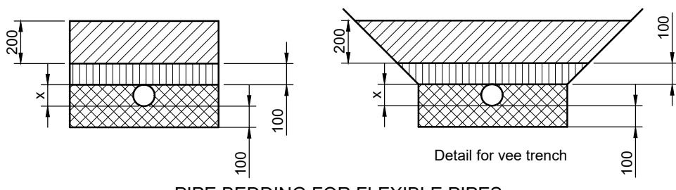
PIPE BEDDING FOR FLEXIBLE PIPES
