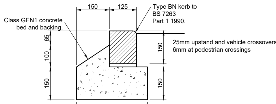
BN KERB DETAIL (Scale 1:10)
