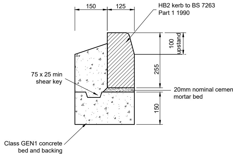
HB2 KERB DETAIL (Scale 1:10)
