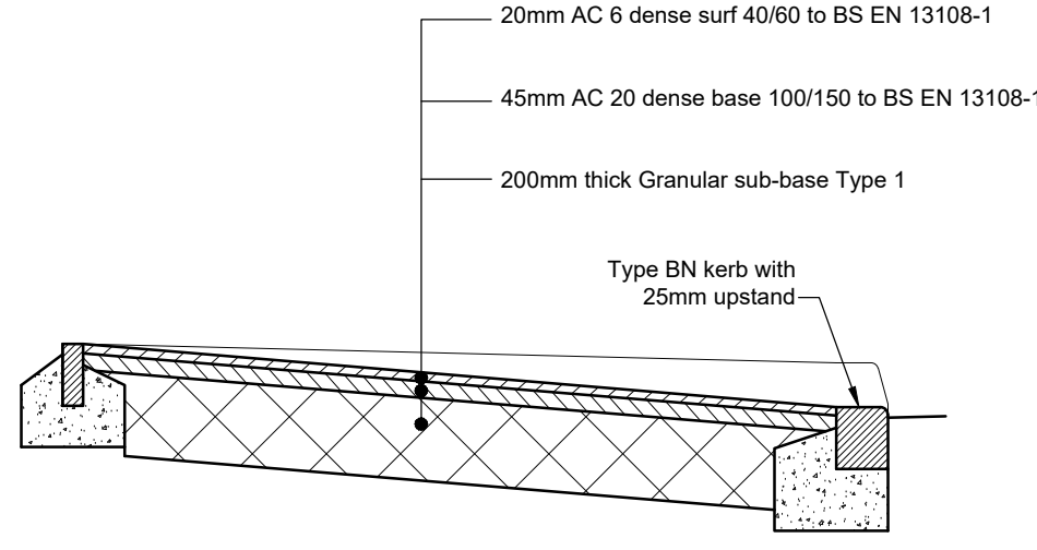
TYPE D - ASPHALT CONCRETE VEHICULAR CROSSOVER CONSTRUCTION (Scale 1:20)
