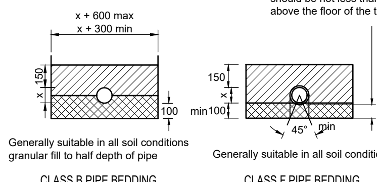
CLASS B PIPE BEDDING
