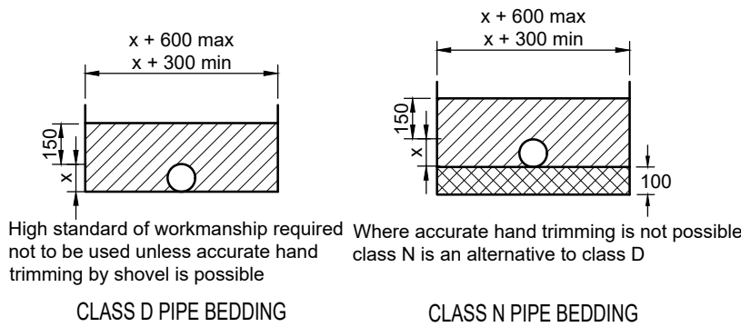
CLASS N PIPE BEDDING
