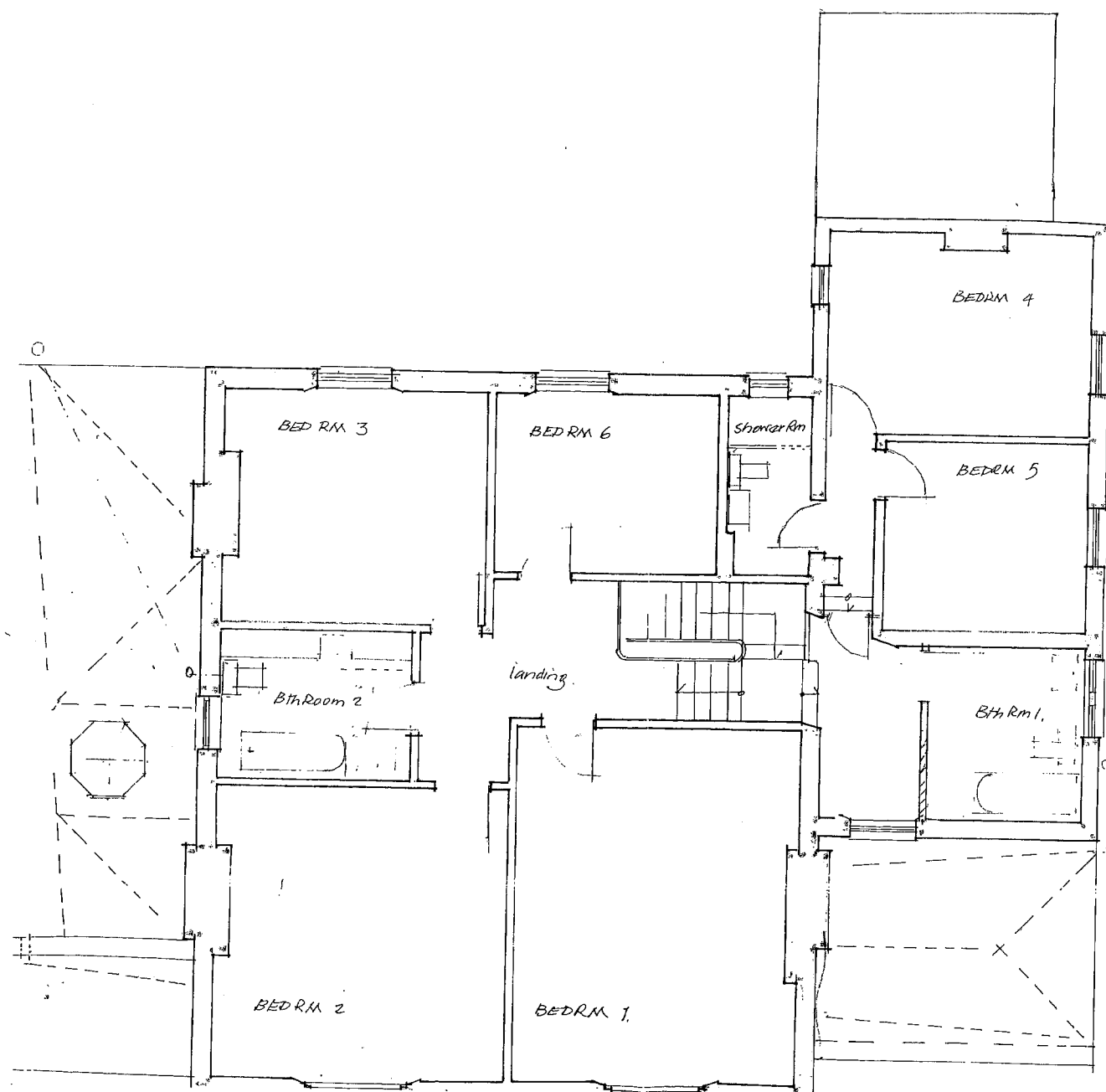
EXISTING FIRST FLOOR 1:100 @ A3
