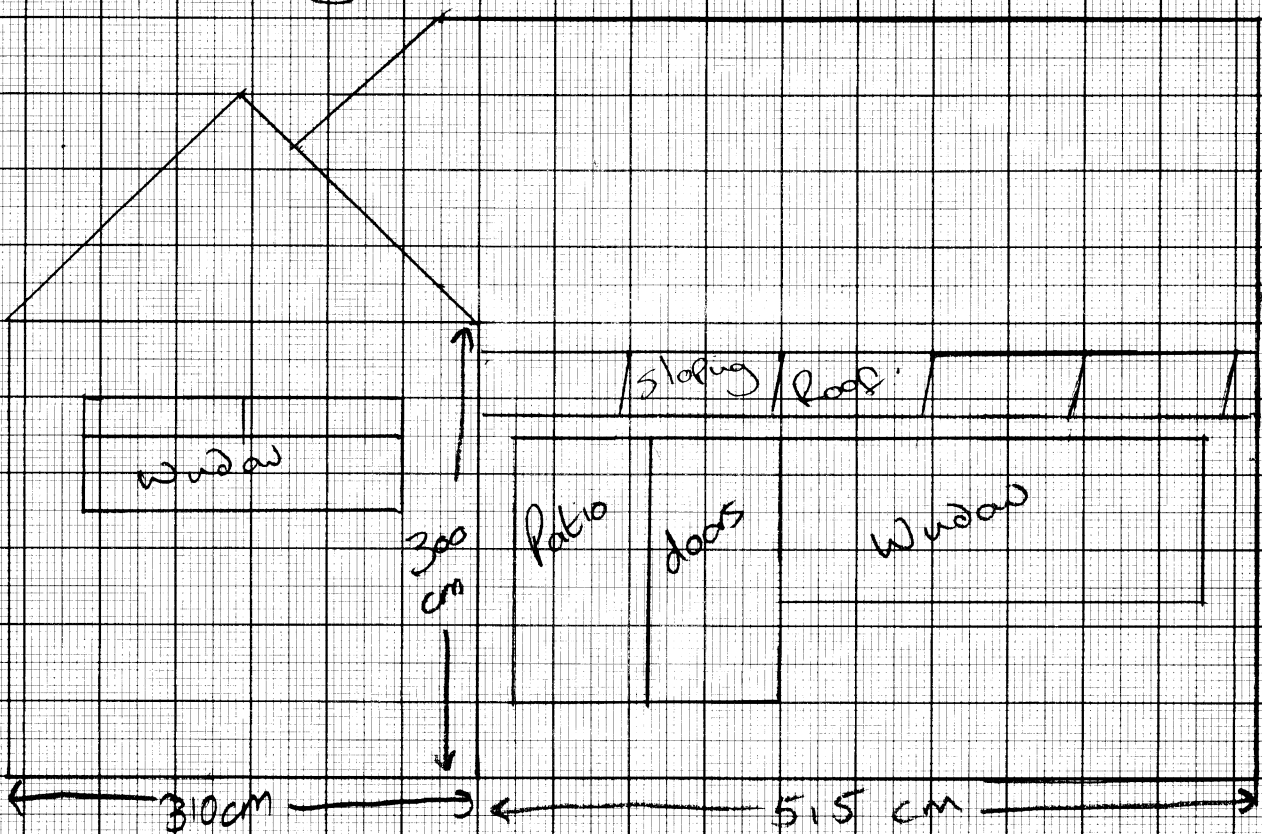
Existing rear view
