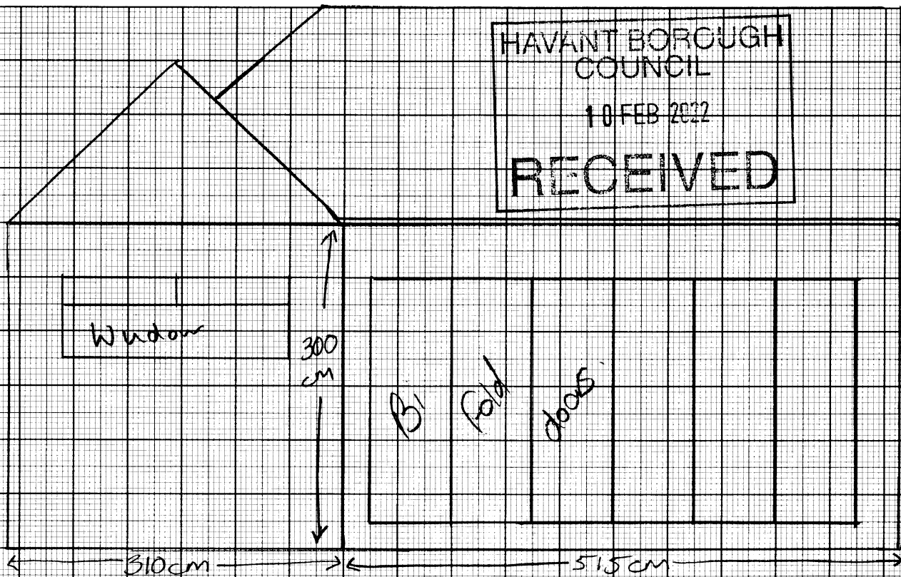
Proposed rear view
